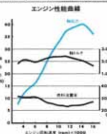
ENGINE PERFORMANCE CURVE
